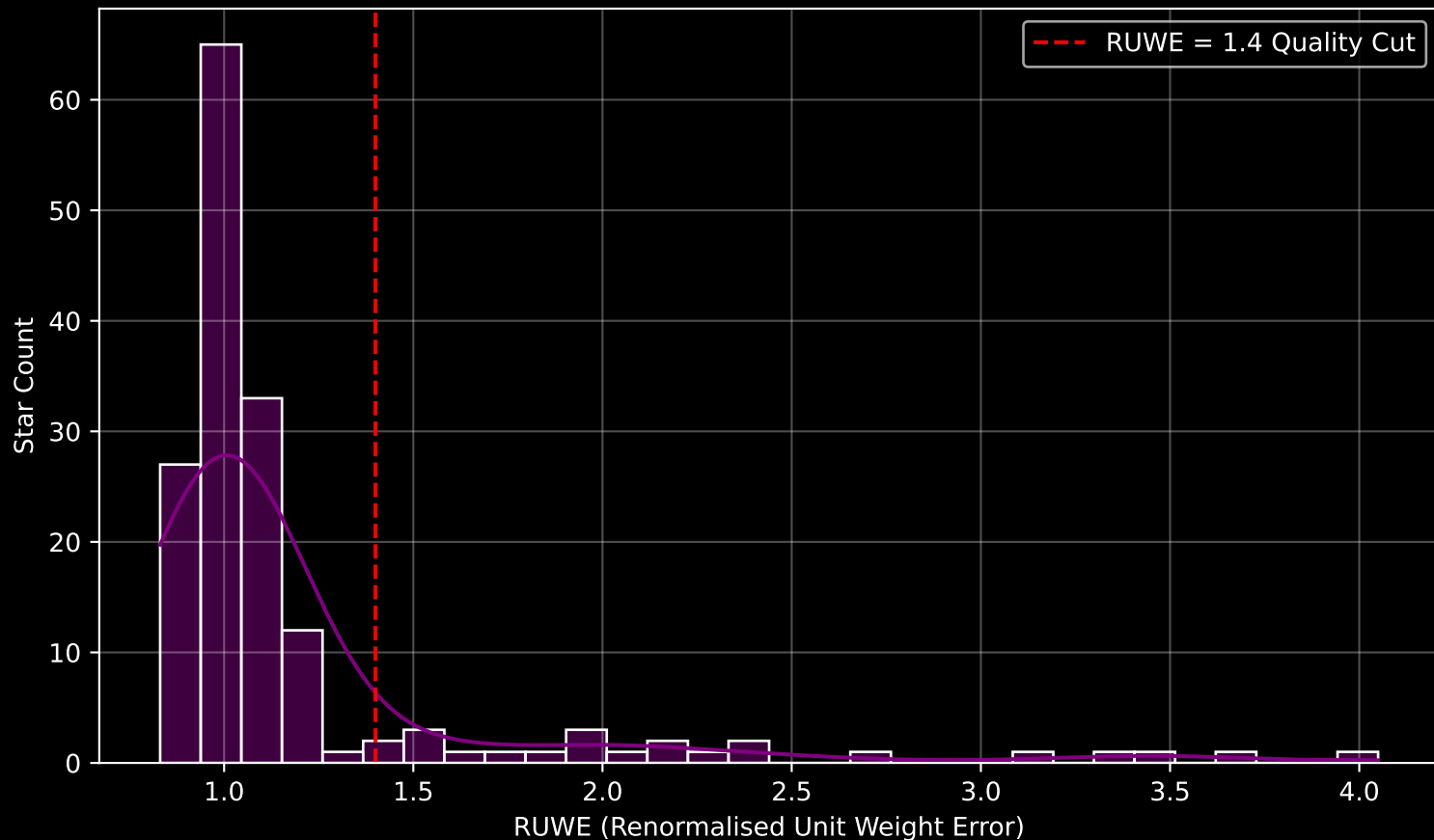
GAPOGEE DR17 Field [050+40_MGA] RUWE Distribution (n= 161)
