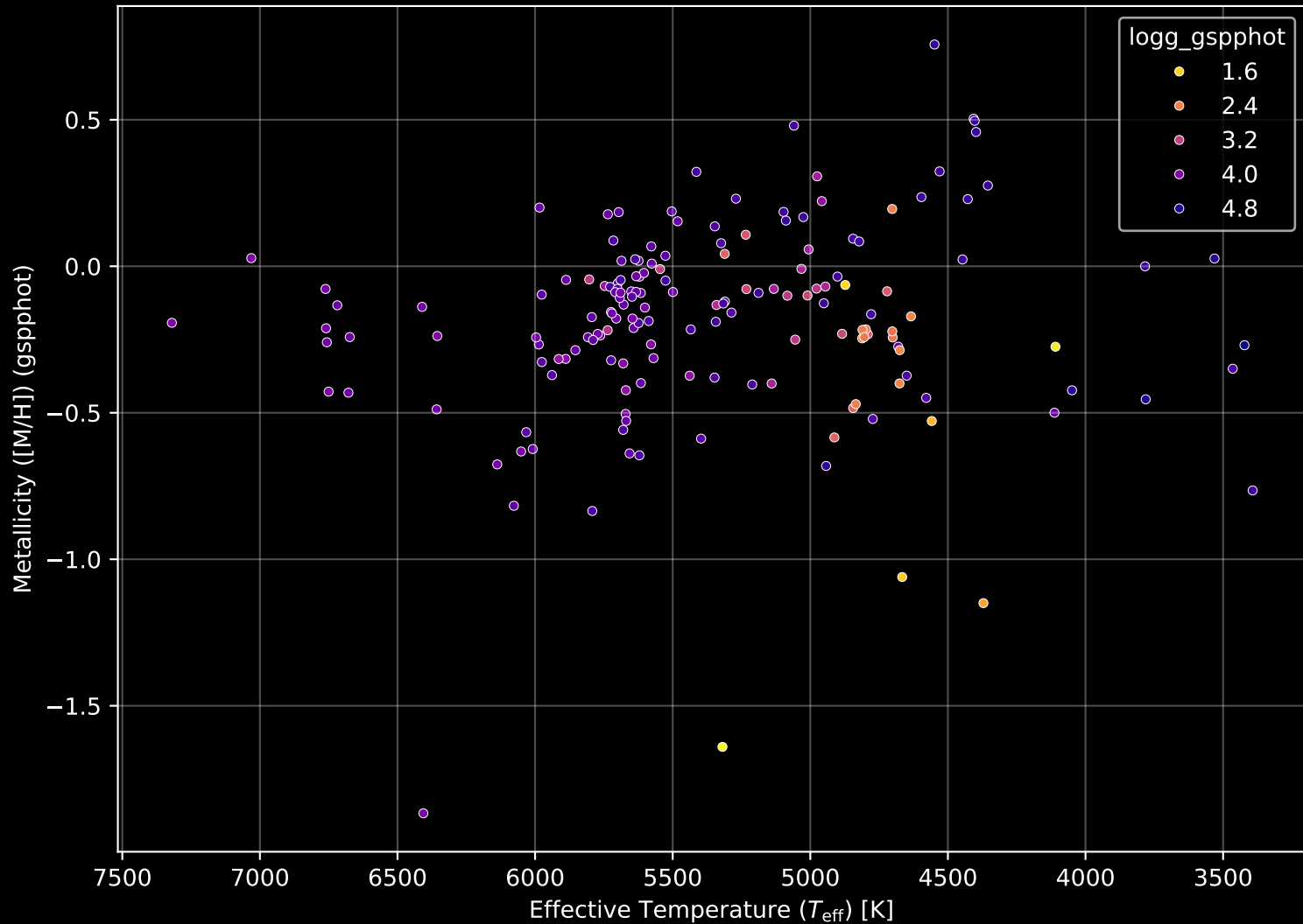
APOGEE DR17 Field: [050+40_MGA] Stellar Population Parameters (n= 167)
