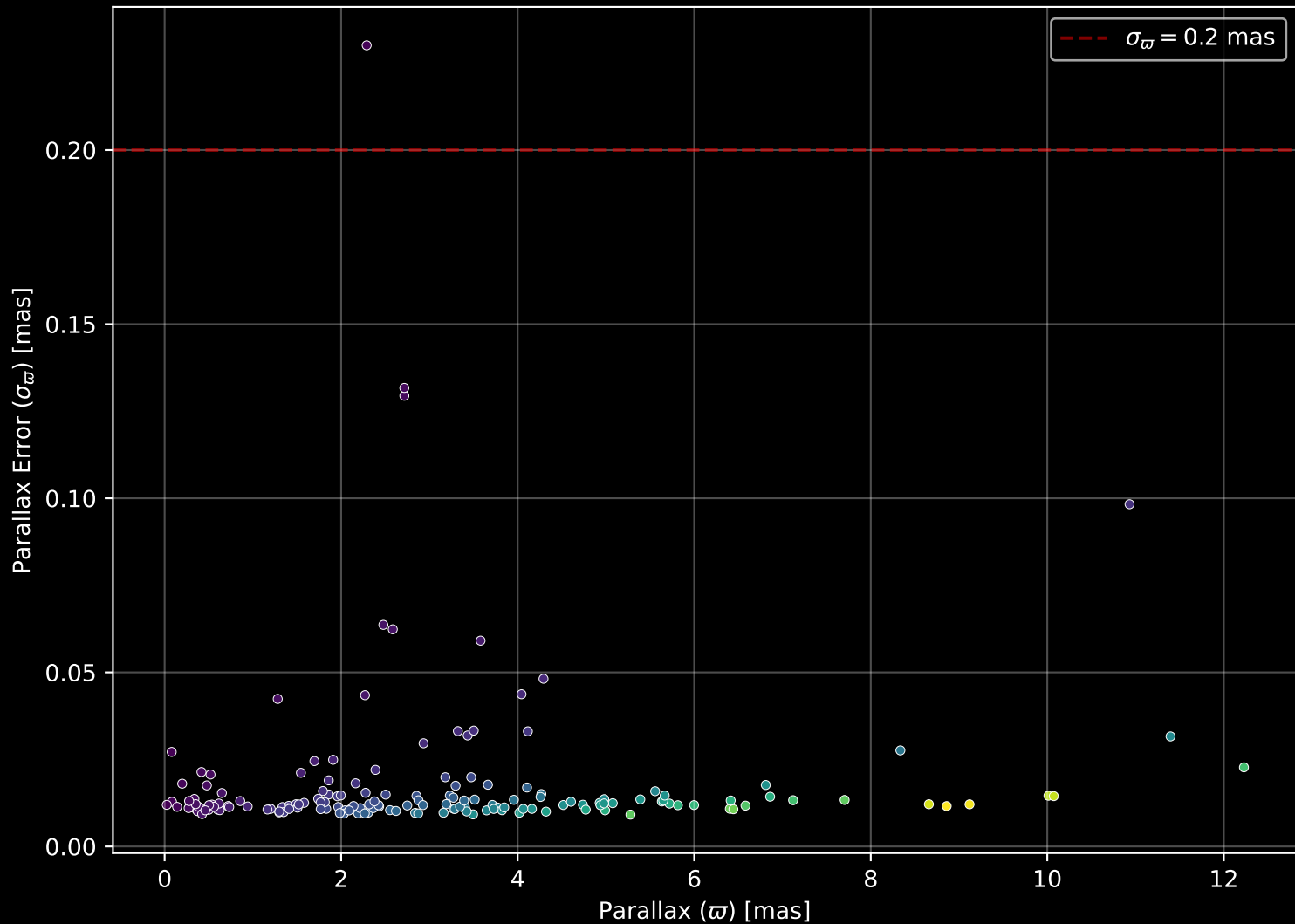
APOGEE DR17 Field: [050+40_MGA] Parallax Quality (n= 167)
