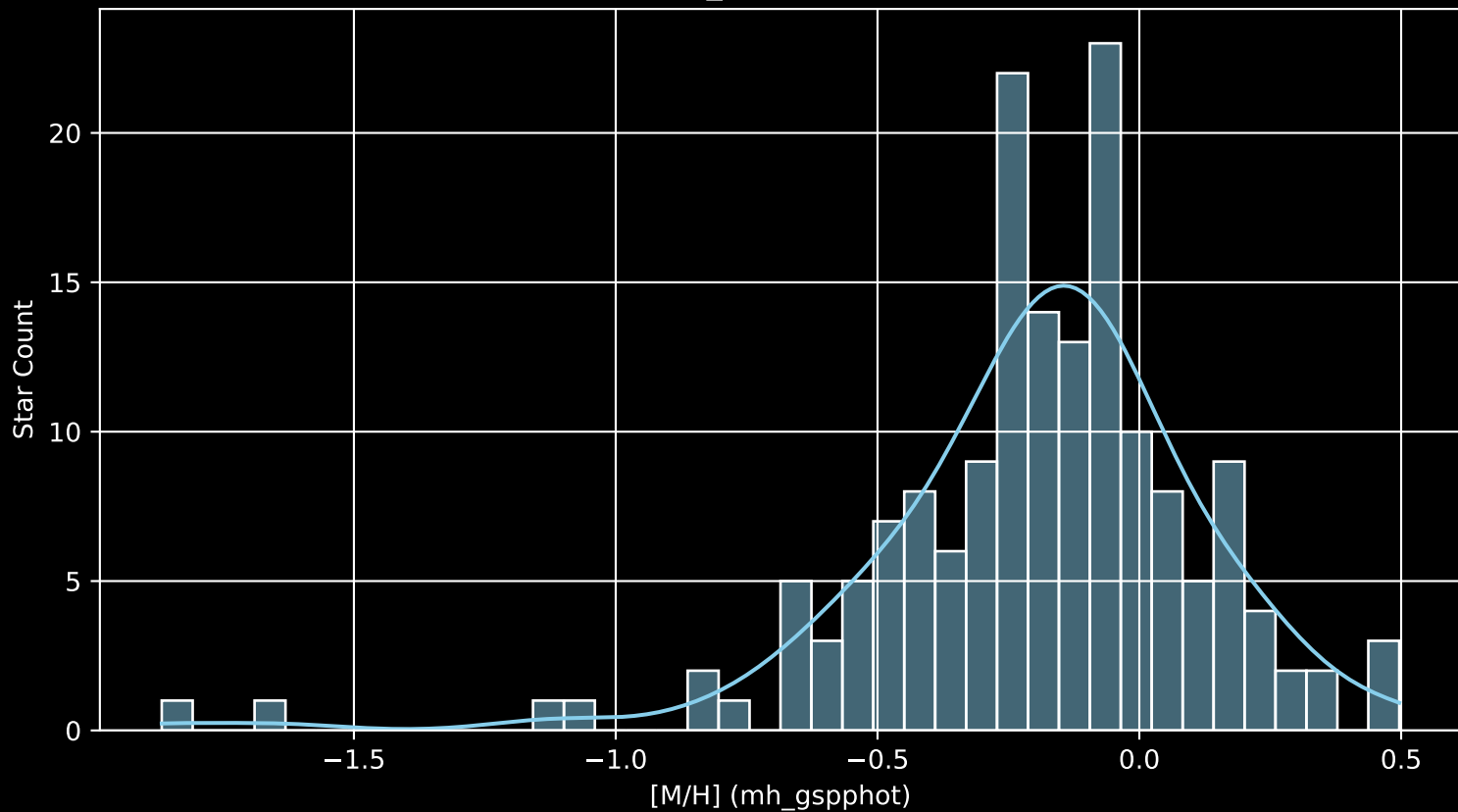
APOGEE DR17 Field: [050+40_MGA [M/H] (mh_gspphot) (n= 165)
