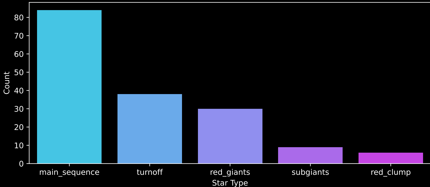
APOGEE DR17 Field: [050+40_MGA] Count plot of Star Type
