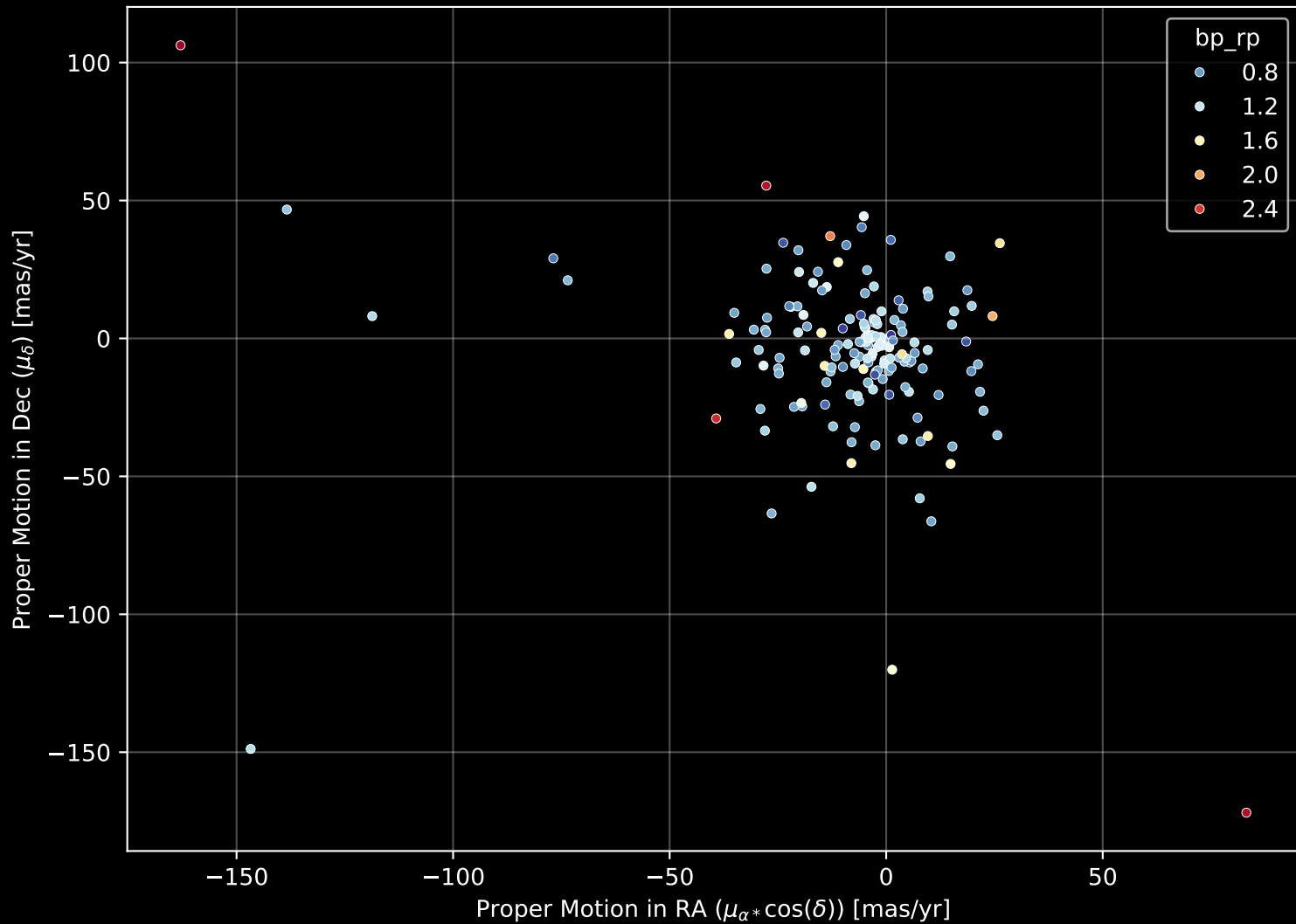
APOGEE DR17 Field: [050+40_MGA] Proper Motion Diagram (n= 167)
